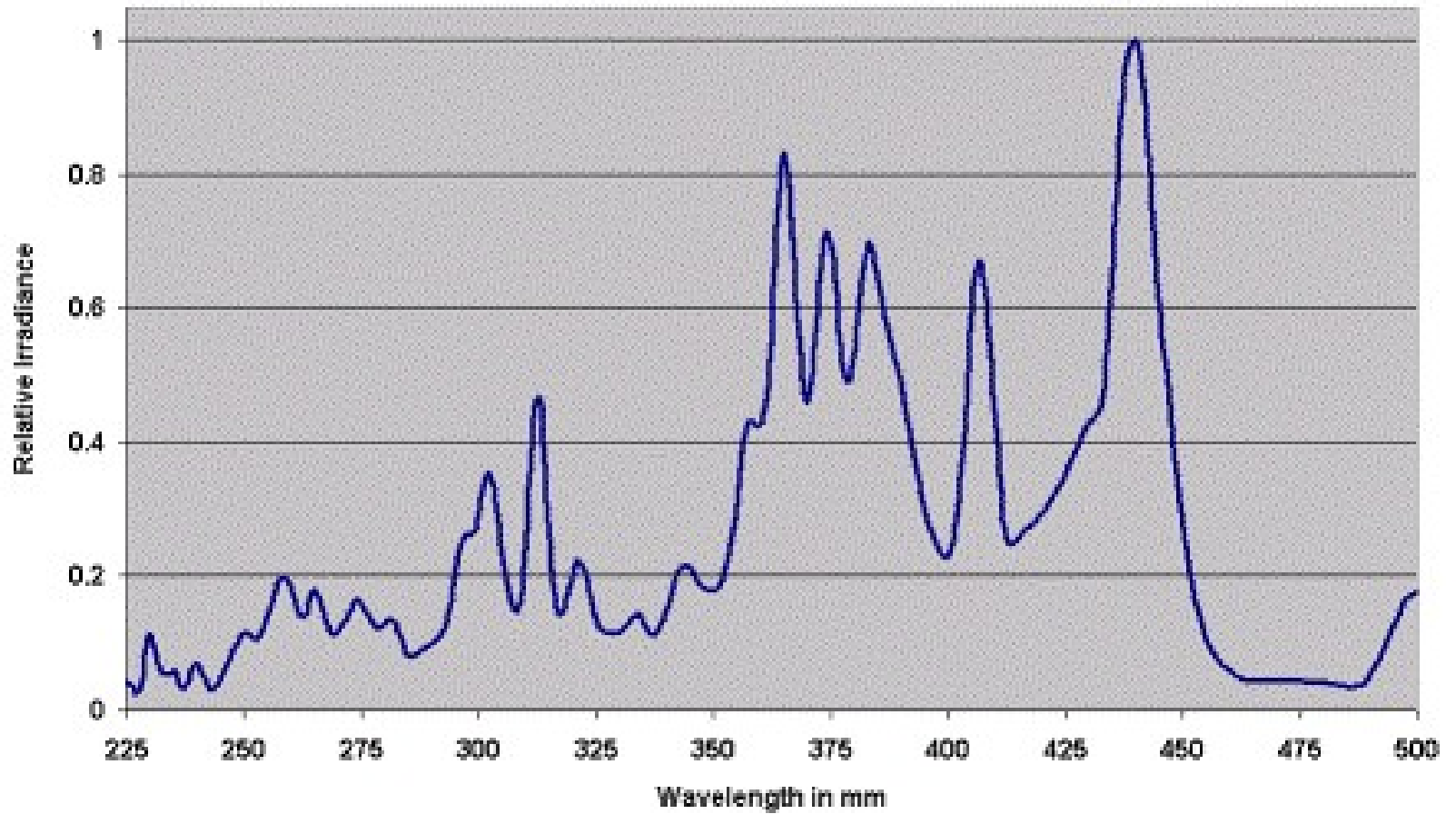
Spectral Output of Electroless D Lamp
