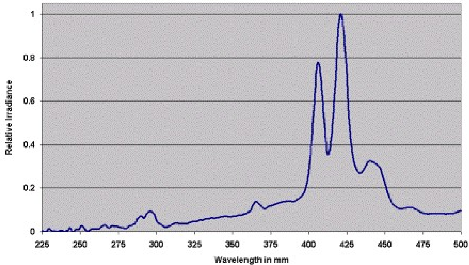
Spectral Output of Electroless V Lamp
